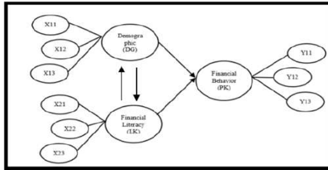
Figure 2. Path Diagram
